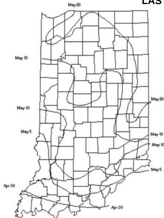
10% Probability for Frost (32°F) After the Date
