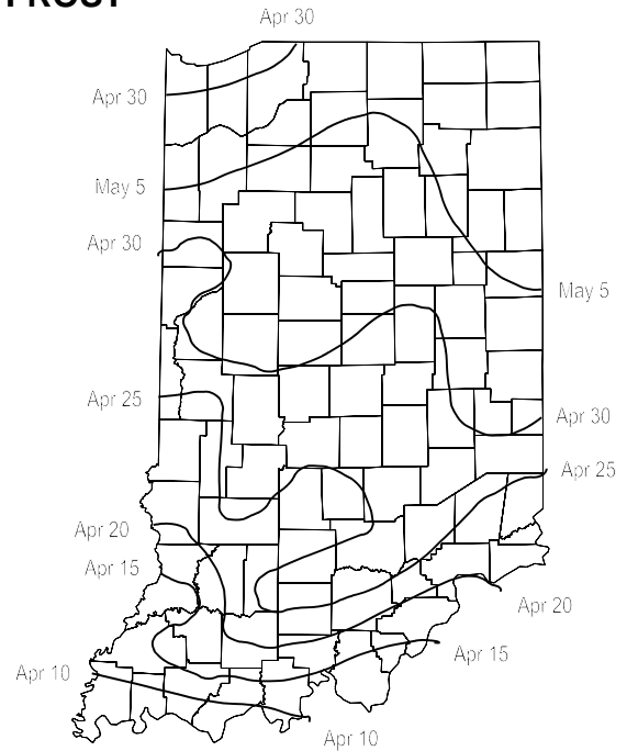
50% Probability for Frost (32°F) After the Date
