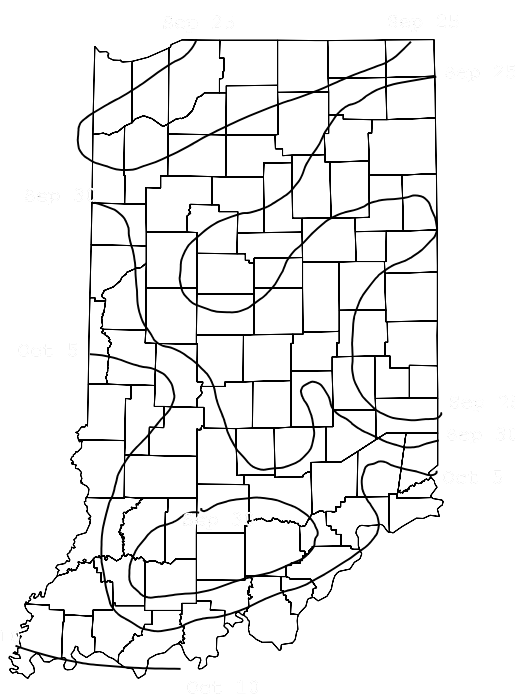
10% Probability for Frost (32°F) Before the Date
